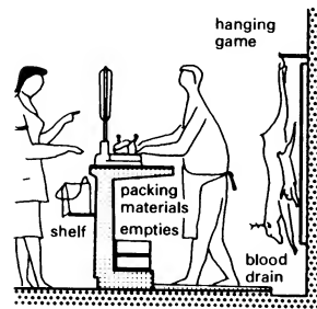
4 Solid counter with marble or tile facing
